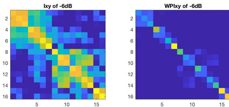
Fig. 2: Heatmaps of the confusion matrix in M&N for a SNR of -6\text{dB} for different preprocessing. Left: pointwise mutual information. Right: weighted pointwise mutual information.
