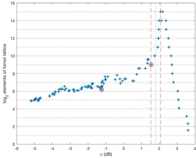
(a) Tomoi count of I(\varphi) vs. \varphi(\text{dB})
