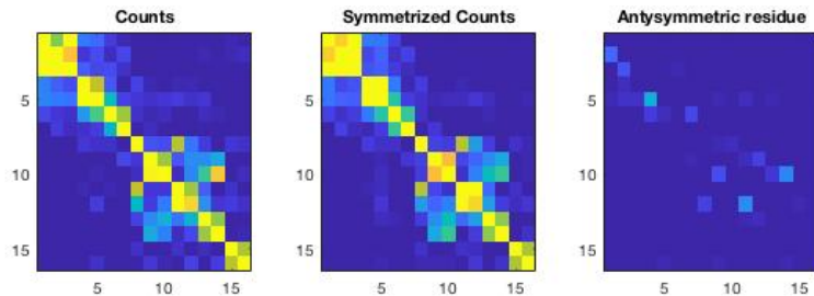
Fig. 1: Heatmaps of the count confusion matrix in M&N for a SNR of -6\text{dB} . Left: count matrix; C center: symmetrized count matrix C_S ; right: antisymmetrical residue C_A .
